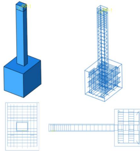
Fig. 3 Finite element idealization (Geometry and reinforcement)
