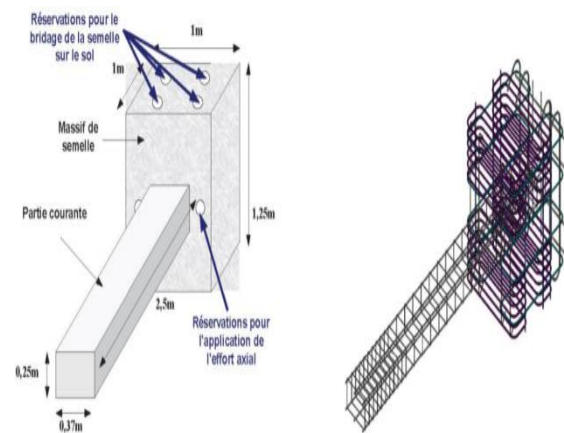
Fig. 1 Geometry and reinforcement of the sample used in the present Study
