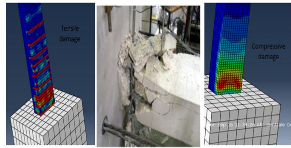
Fig. 6 Comparison of the local failure
