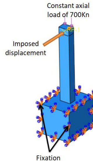
Fig. 4 Loading and boundaries condition
