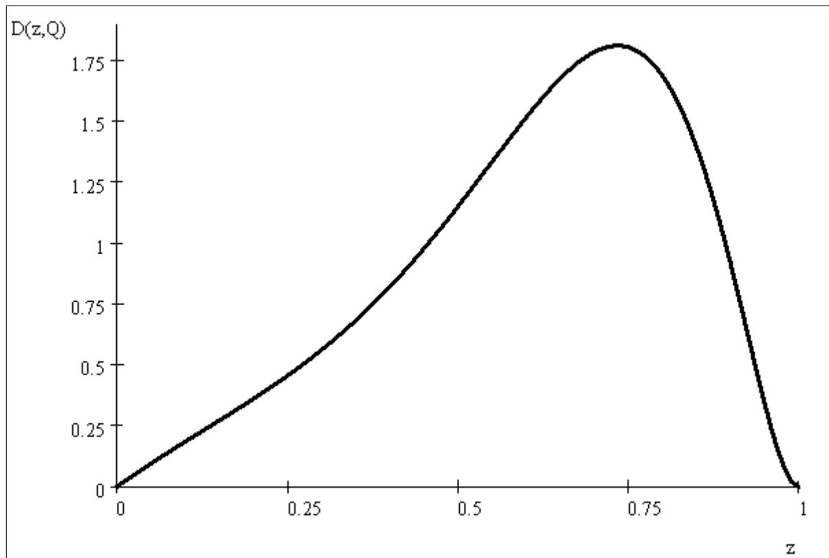
Fig. 7. Fragmentation function at T = 0 .(J.P.Ma result).
