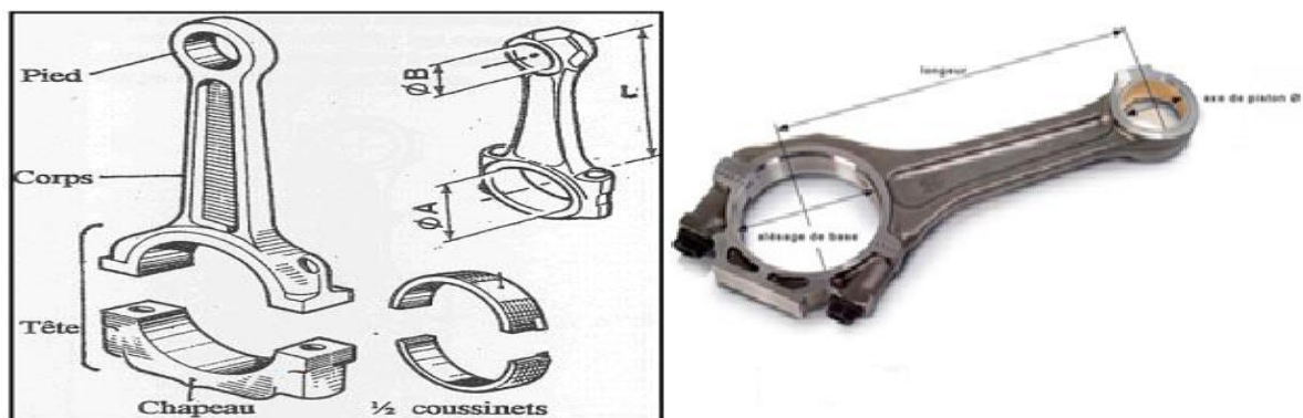
Figure I.7: la bielle.
