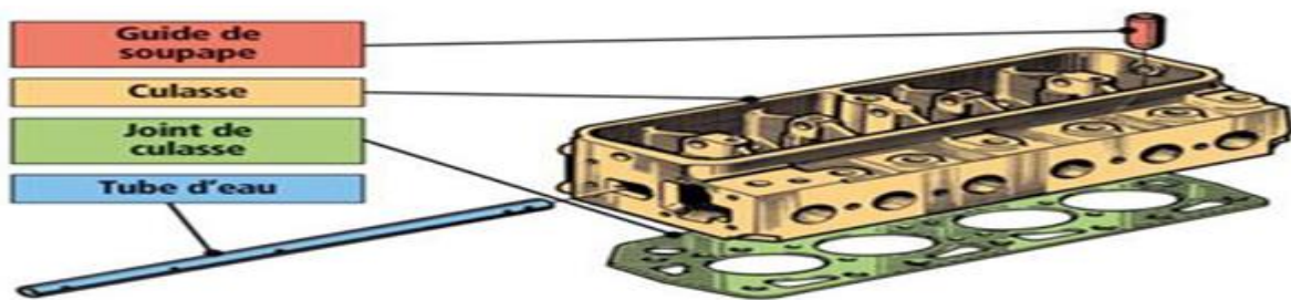
Figure I-4: Culasse
