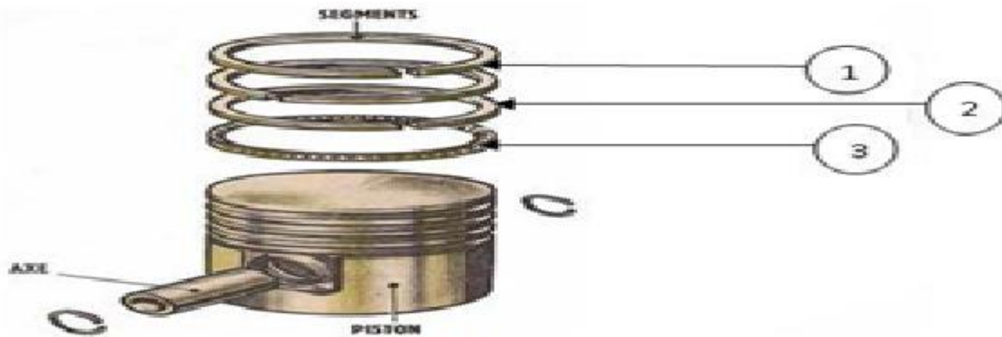
Figure I- 6: Piston
