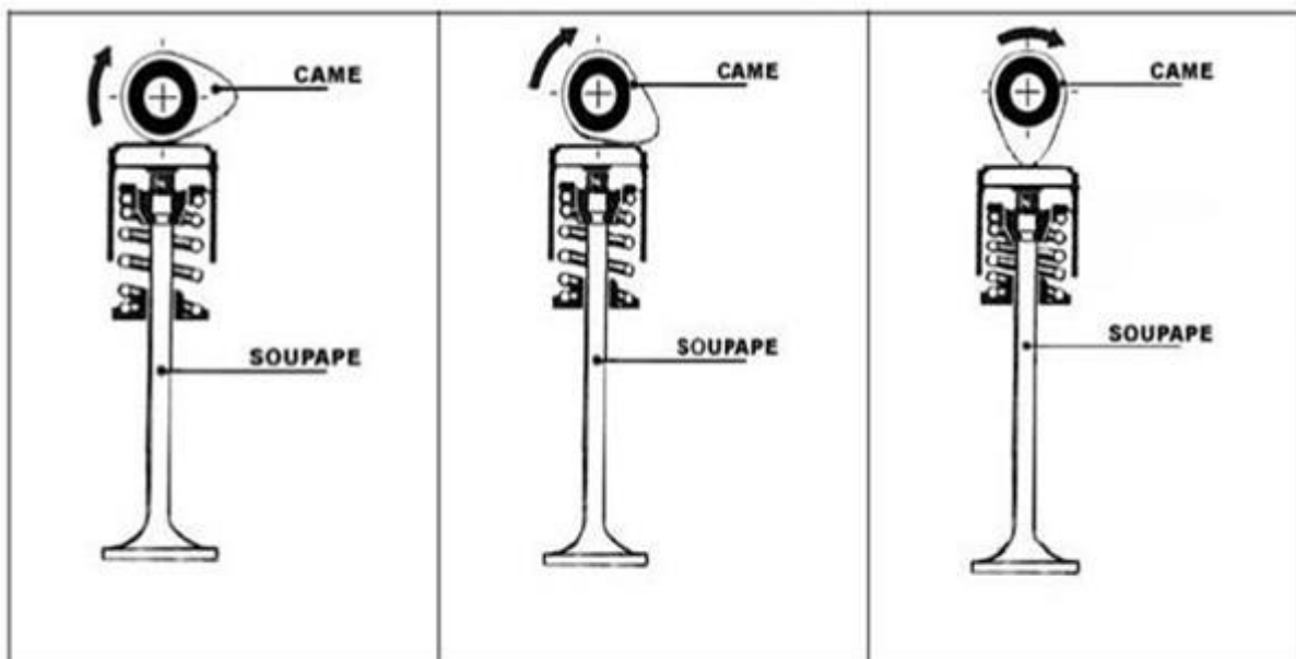
Figure I.10 : les soupapes.
