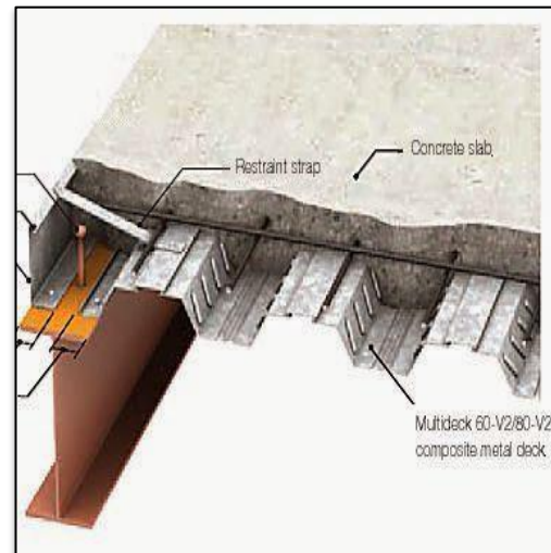
Figure 199 : plancher collaborant Source : Google Image
