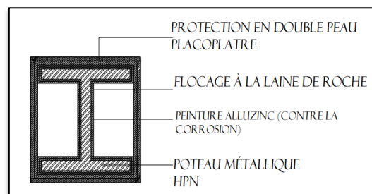
Figure 195: poteau métallique HPN.
