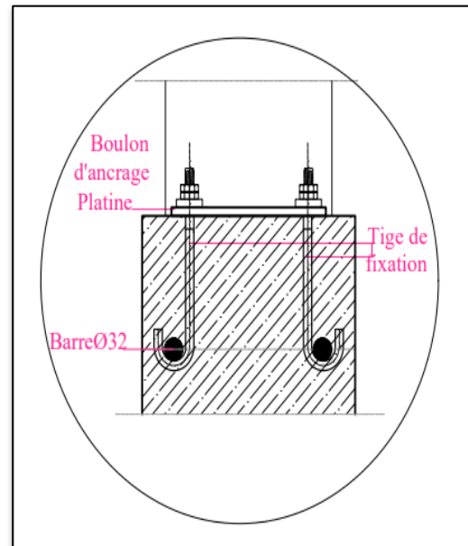
Figure 213: assemblage poteau fondations Source : Autocad
