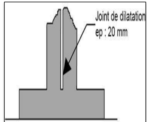
Figure 187 : Figure 107 Joint de dilatation. Source : http://www.Google image.com
