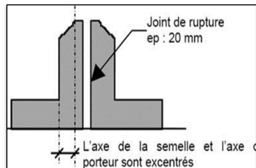
Figure 188 : Figure 107 Joint de rupture. Source : http://www.Google image.com
