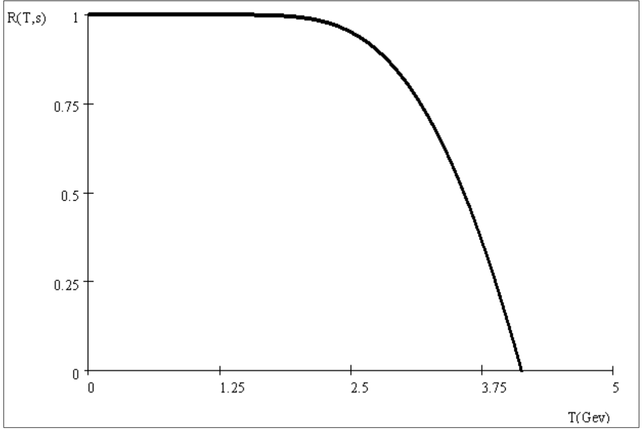
Fig. 5. Ratio of non-parity conserving part versus temperature for pions. c.m energy: \frac{\sqrt{s}}{2} = 10\text{Gev} .
