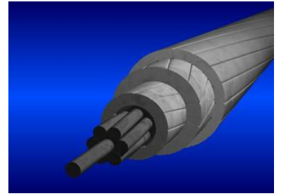
Figure III.10 : câble ACSS
