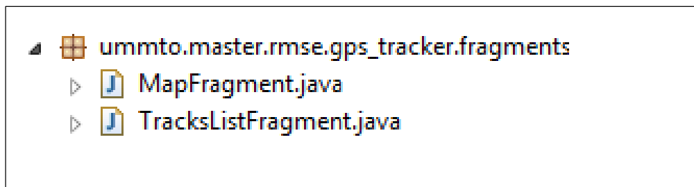
Figure 4.6. Package ummto.mastrer.rmse.gps_tracker.fragments
