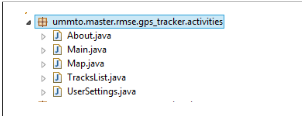
Figure 4.4. Package ummto.mastrer.rmse.gps_tracker.activities
