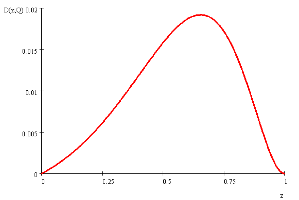
Fig. 6. Fragmentation function D(z, Q) at T = 0 .
