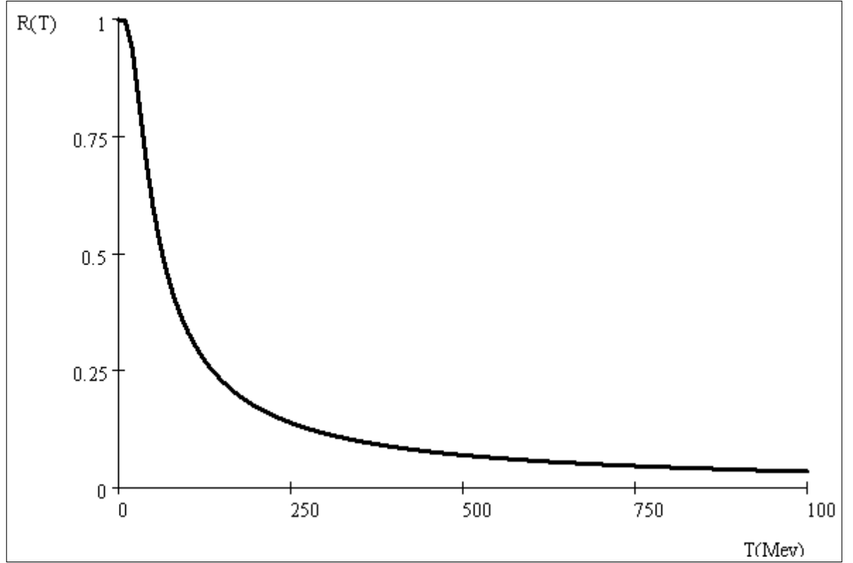
Fig. 4. Differential cross section rate for pion production in e^+e^- annihilation and comparison with the zero temperature case. centre of mass energy: \sqrt{s} = M = m_{\pi^\pm} = 140 \text{ Mev} and chemical potential: \mu = 0 \text{ Mev} .
