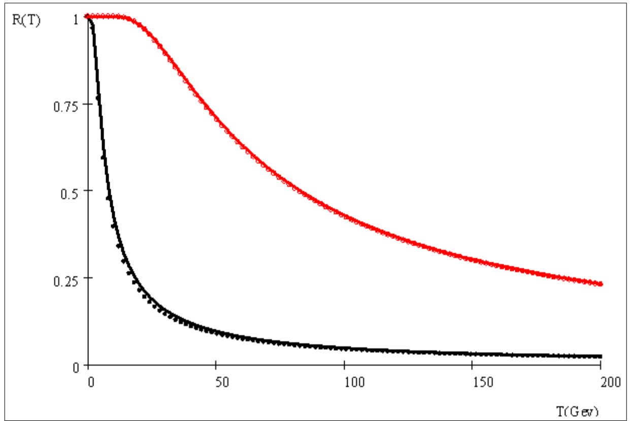
Fig. 2. Black continuous curve: \mu = 0 Mev. Black dotted curve : \mu = 400 Mev. \sqrt{s} = 10 Gev. Red continuous curve : \mu = 0 Mev. Red circle curve : \mu = 400 Mev. \sqrt{s} = 100 Gev. (total cross section rate for e^+e^- annihilation in the Z_0 channel)
