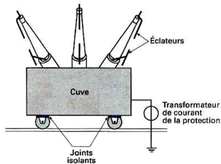
Figure (III-7) : Protection masse-cuve
