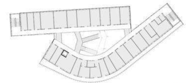
Plan de R+1 / First floor
