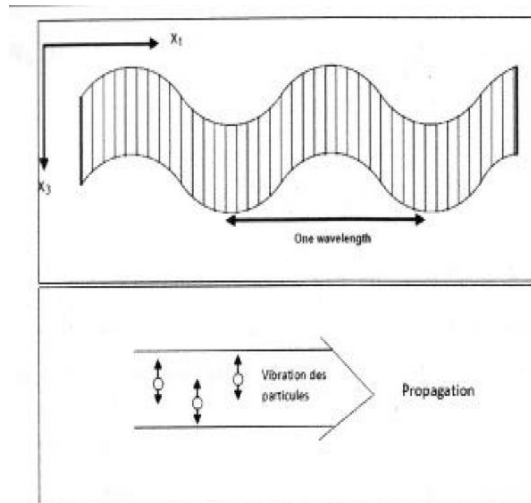
Figure I.17 Ondes transversales
